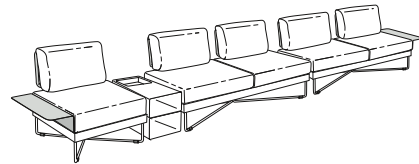
art. 9833 oval sunloom cm 455x83x83h (Hs. cm 26+15)
